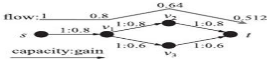
Fig. 4. Generalized maximum flow
