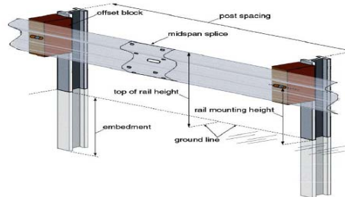
Figure 1: Use of midspan splices and offset blocks in a MGS (Ochoa, C & Ochoa, T, 2011).
