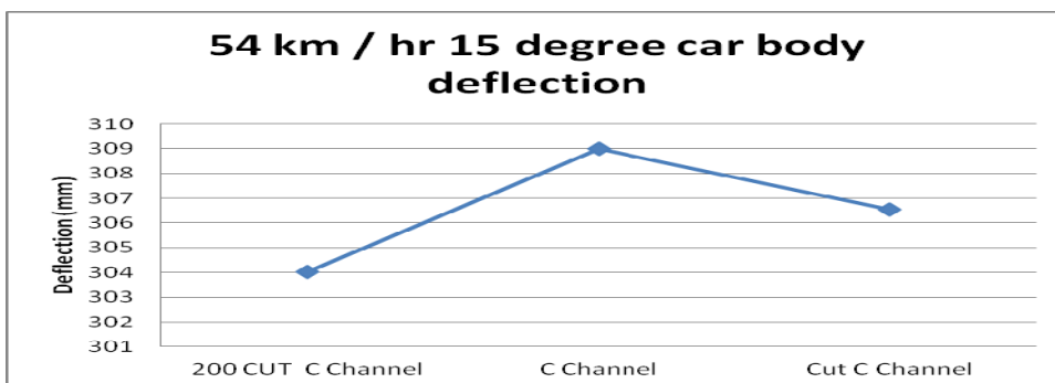
Figure 7: 54 km/hr 15 degree car body deflection graph.
