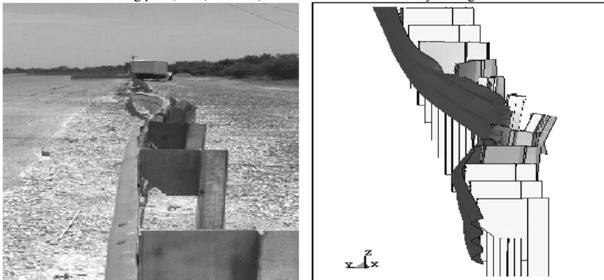
Figure 2: Highway guardrail (a).
