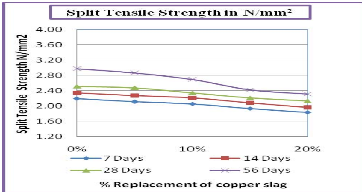
Graph 2: Split Tensile Strength of M-25 Mix cubes at different curing stages.
