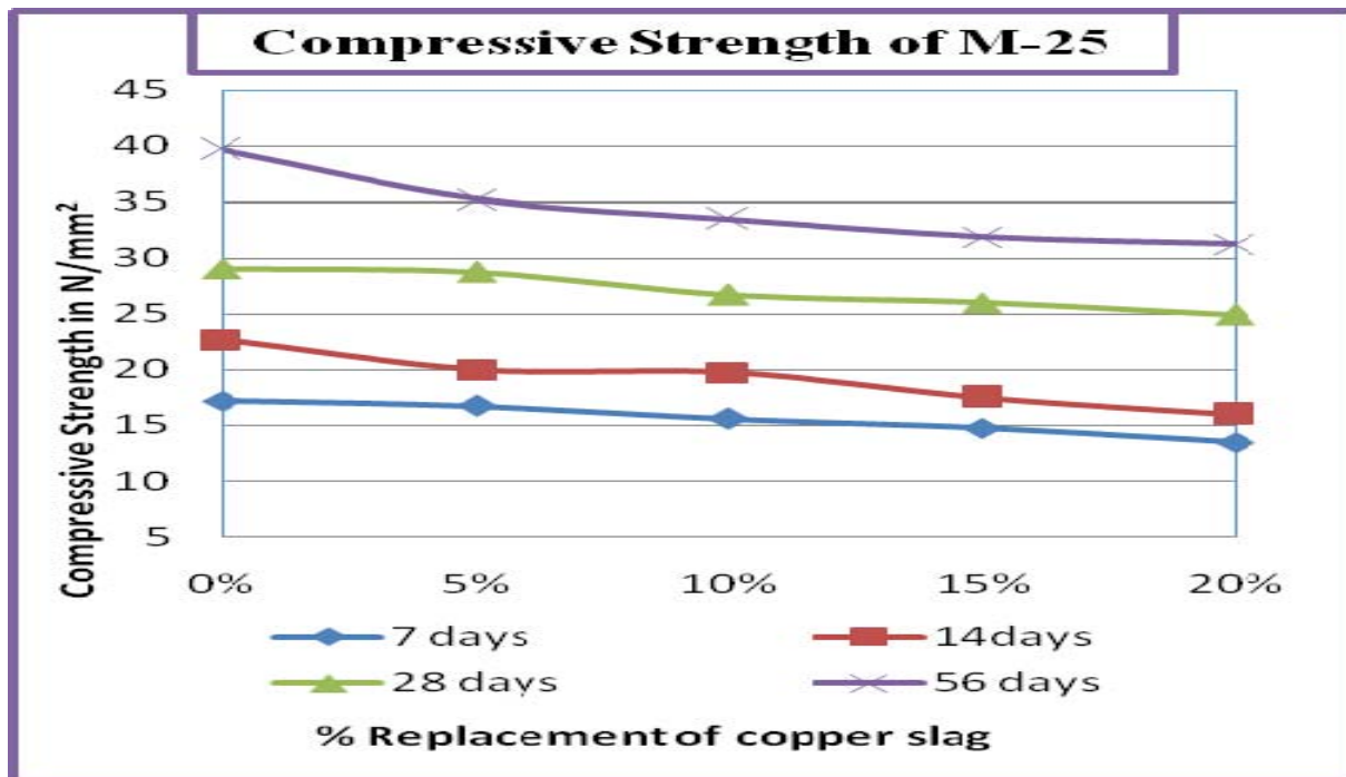
Graph 1: Compressive Strength of Concrete M-25.
