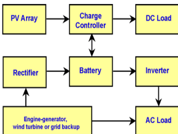
Fig 4: Diagram of photovoltaic hybrid system.
