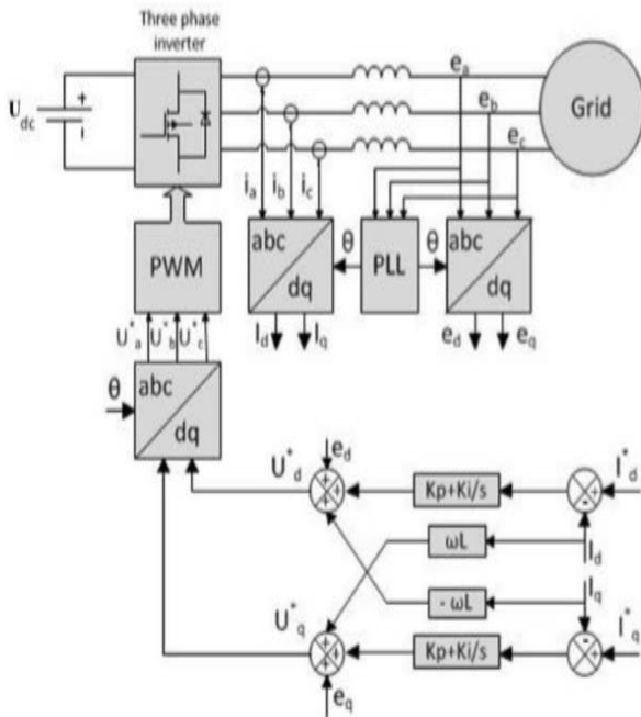
Figure 8: Block diagram of Synchronous reference frame control.
