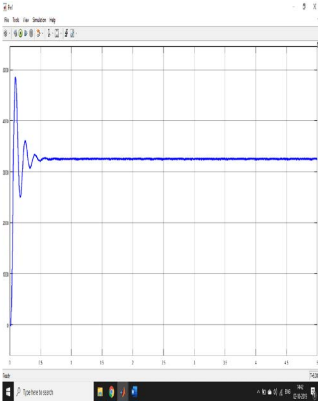
Figure 4.7: Wind farm power with SRF control.
