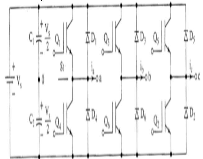
Figure 7: Three Phase Voltage Source Inverter Topology.
