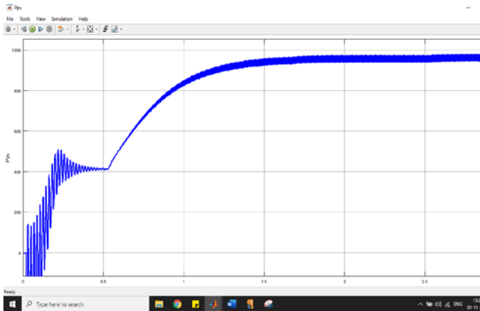
Figure 4.2: Power output from PVA without SRF control.
