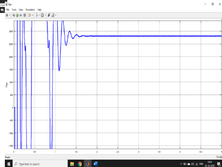
Figure 4.6: PVA power with SRF control.
