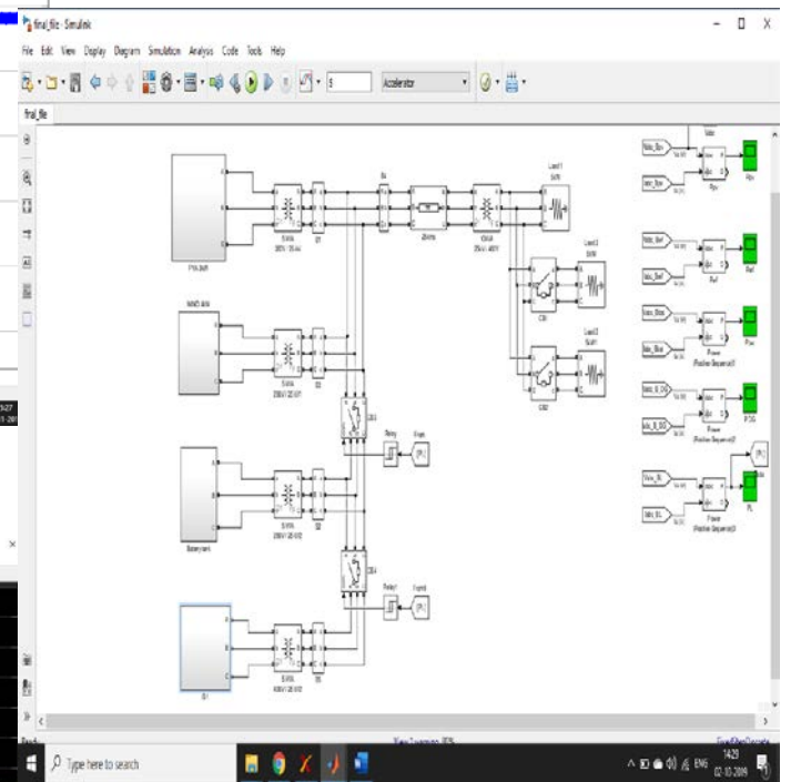
Figure 4.5: Proposed test system with battery and DG connected to grid with SRF control.
