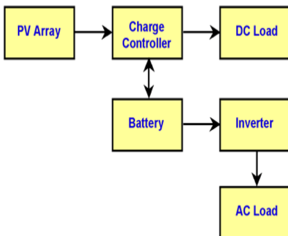
Fig 3: Diagram of stand-alone PV system with battery storage powering DC and AC loads.
