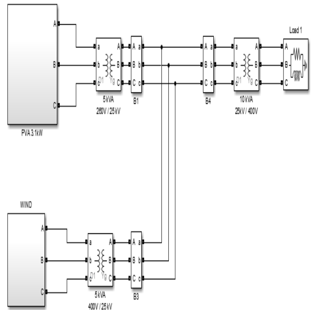
Figure 4.1: Only wind and solar system connected grid without SRF control.
