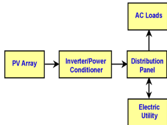
Fig 1: Diagram of grid-connected photovoltaic system.
