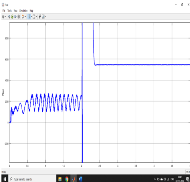
Figure 4.8: Battery power with SRF control.
