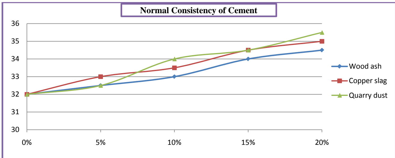
Fig 3: Normal Consistency of Cement.
