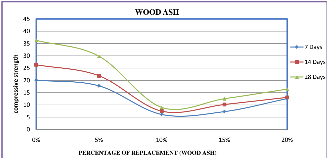
Fig 5: Compressive Strength of M25 Grade Contain of Wood Ash
