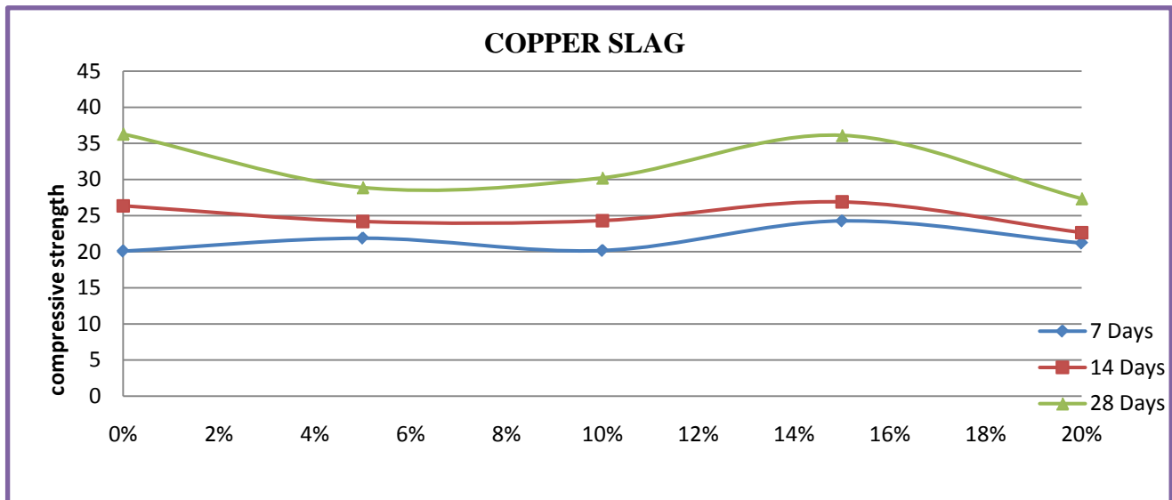
Fig 6: Compressive Strength of M25 Grade Contain of Copper Slag.
