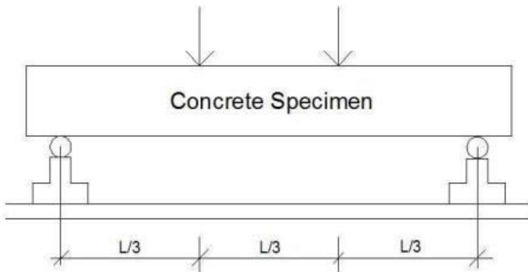
Fig 1: Arrangements of Third Point Loading.
