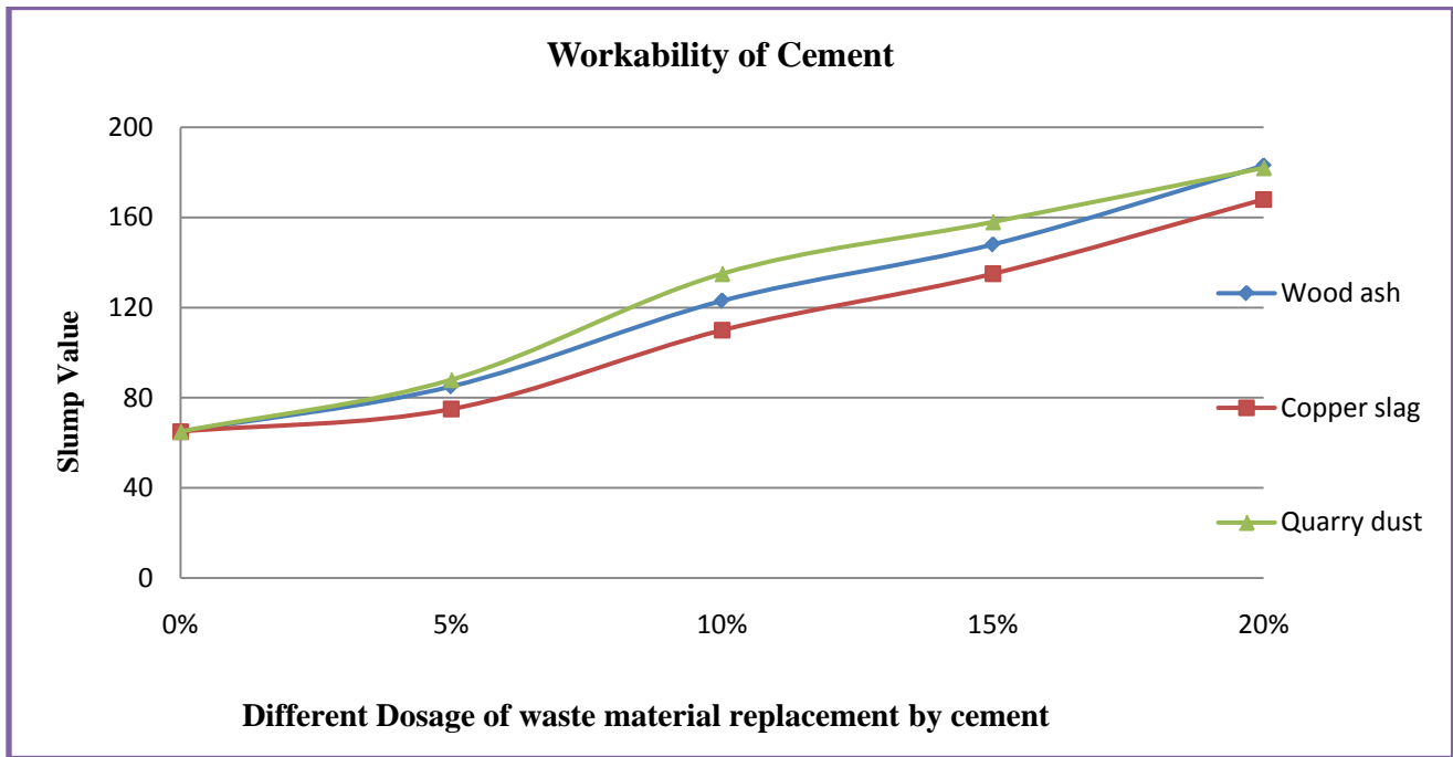
Fig 4: Slump Values of Different Waste Material.
