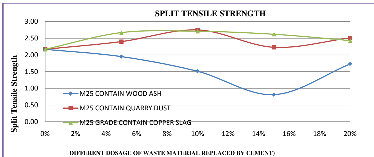
Fig 8: Split Tensile Strength.
